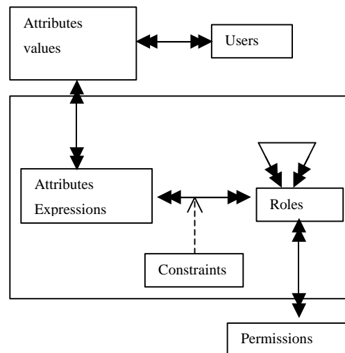
Figure 1: RB-RBAC model
